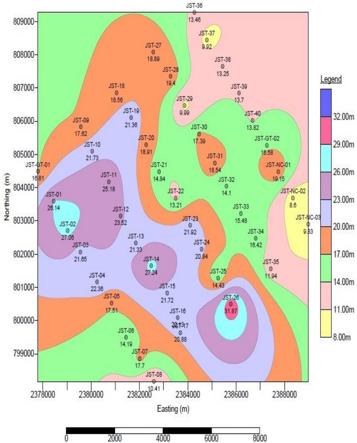
Figure-6.1: Isopach Map Showing Cumulative Coal Thickness of Drilled Boreholes , Block-XII Janib Ali Shah Jo Tar (DRD), Thar Coalfield Sindh Pakistan
