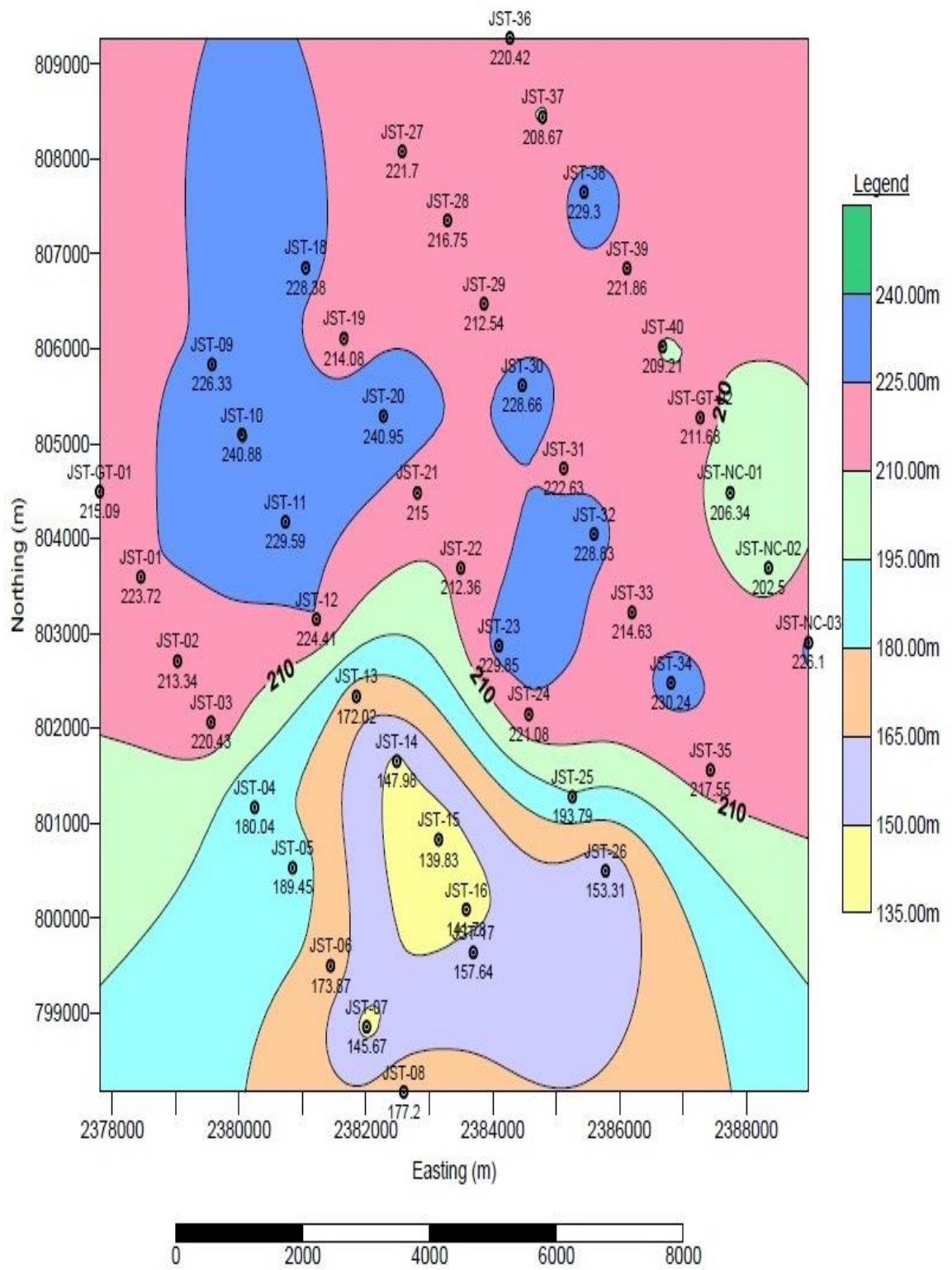
Figure-6.5: Isopach Map Showing Overburden Thickness of Drilled Boreholes, Block-XII Janib Ali Shah Jo Tar(DRD), Thar CoalField Sindh Pakistan
