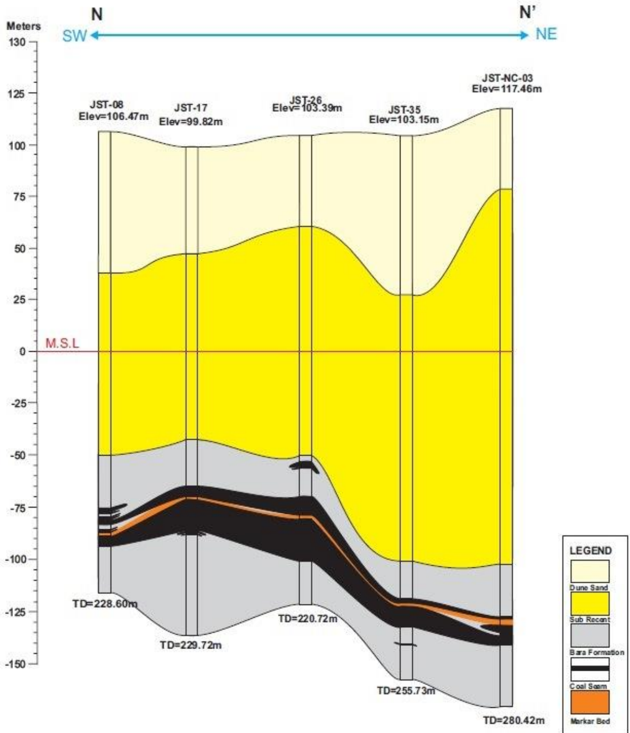
Cross-section Along Line N-N', Block-XII, Janib Ali Shah Jo Tar (DRD), Thar Coal Field, Sindh, Pakistan
