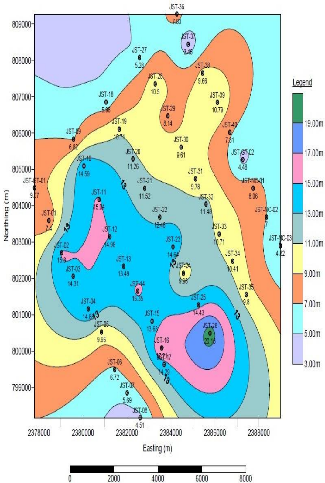
Figure-6.2: Isopach Map Showing Main Seam Thickness of Drilled Boreholes, Block-XII Janib Ali Shah Jo Tar(DRD), Thar CoalField Sindh Pakistan
